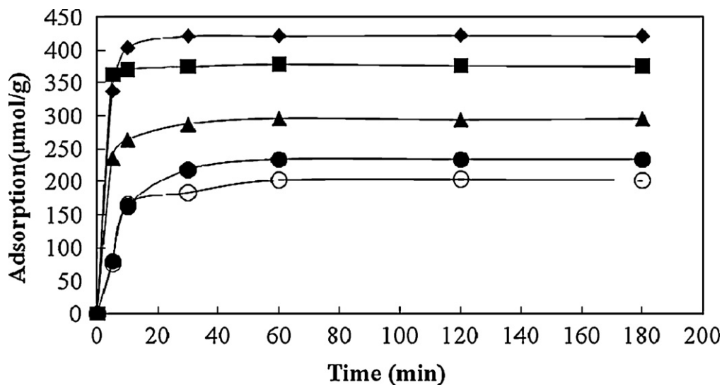
Fig. 8. Capacities of the PUF/diatomite/dispersed-MWCNTs for adsorption of the targeted dyes of acridine orange (◆), methylene blue (■), ethidium bromide (▲), eosin Y (●), and eosin B (○), respectively.
