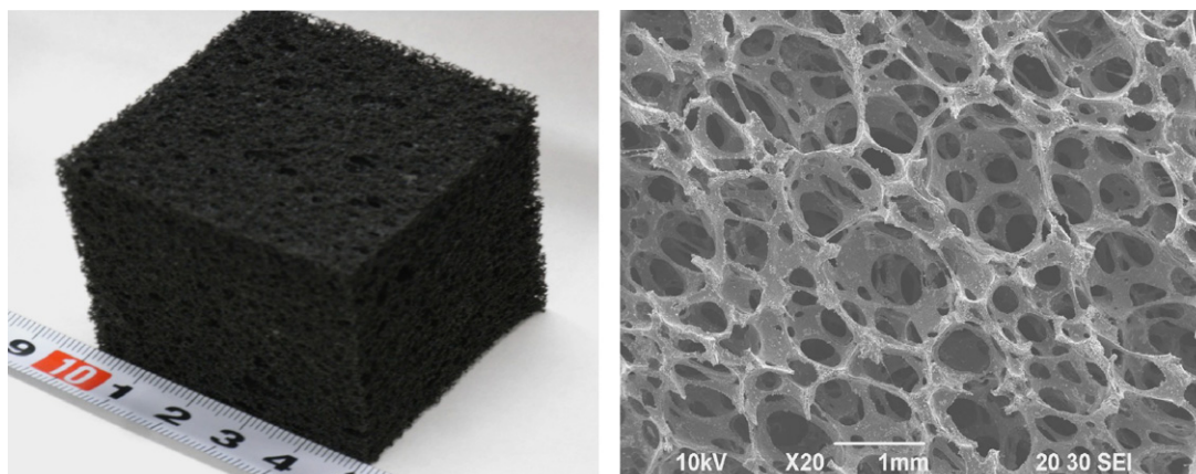
Fig. 7. Photo (left) and SEM observation (right) of the macro-sized, foam-like, ternary CNT-based adsorbent.
