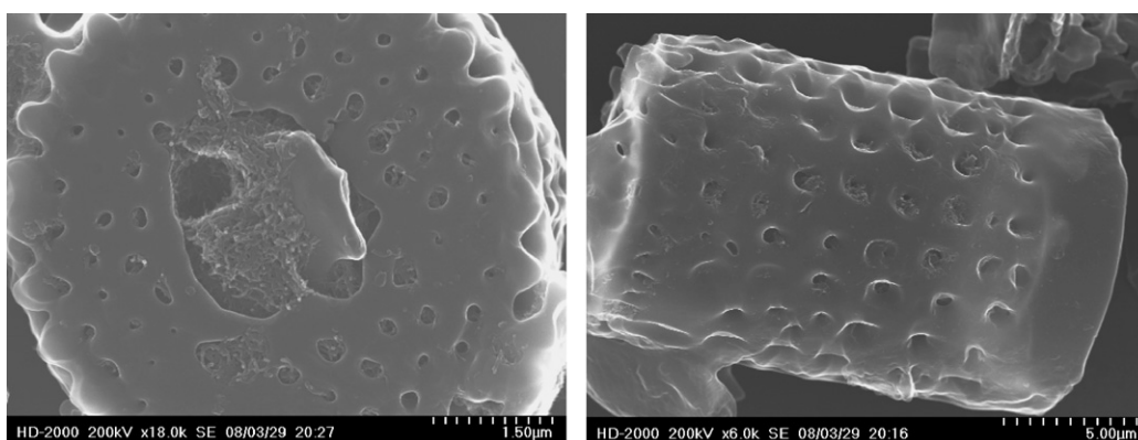
Fig. 3. SEM images of the dispersed-MWCNTs after being packed into the cavities of the diatomite.
