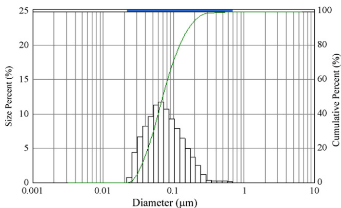
Fig. 1. Dynamic light-scattering size distribution of the dispersed-MWCNTs in the aqueous suspensions.
