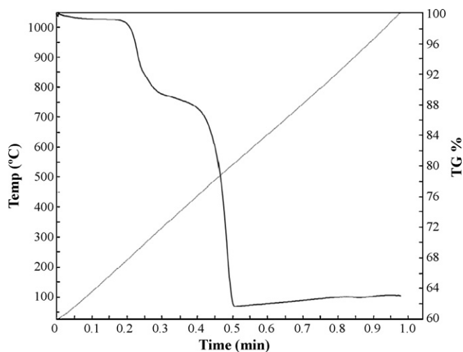
Fig. 4. TG-A measurement of the contents of the MWCNTs in the diatomite/dispersed-MWCNTs.
