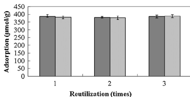
Fig. 9. Three cycles of adsorption/desorption for methylene blue using PUF/diatomite/dispersed-MWCNTs as the adsorbent.
