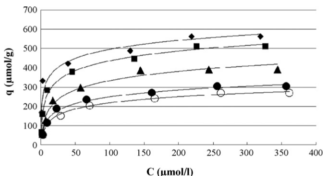
Fig. 10. Langmuir isotherms for sorption of the model dyes by the PUF/diatomite/dispersed-MWCNTs. Dyes are acridine orange (◆), methylene blue (■), ethidium bromide (▲), eosin Y (●), and eosin B (○), respectively.
