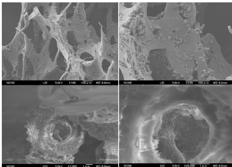
Fig. 6. SEM images of diatomite/dispersed-MWCNTs after being immobilized on the cell walls of PUF through in situ PUF formation. Scale bars: upper pictures: 100 \mu\text{m} ; lower pictures: 1 \mu\text{m} , respectively.
