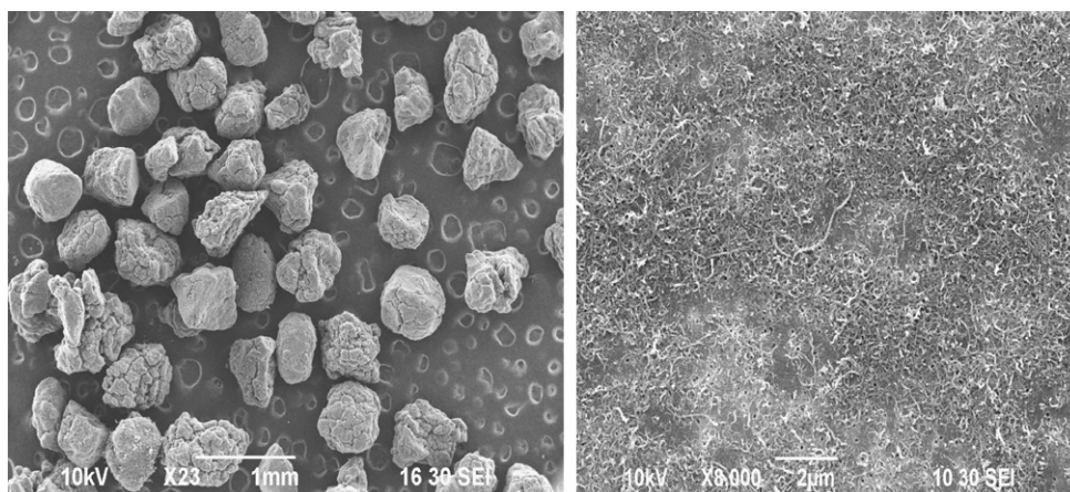
Fig. 2. SEM images of the as-received agglomerates of MWCNTs (left) and the agglomerates after being dispersed into the dispersed-MWCNTs (right).
