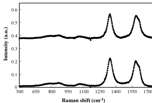
Fig. 5. Raman spectroscopies for the as-received MWCNTs (the CNT-agglomerates, bottom) and, the dispersed-MWCNTs after being packed into the cavities of the diatomite (top).
