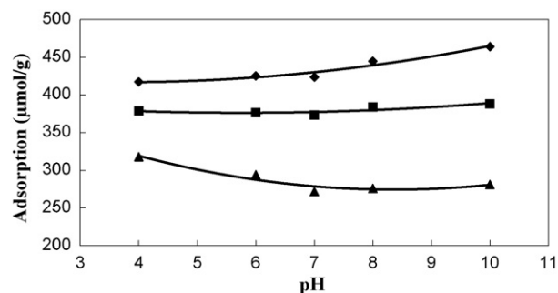
Fig. 11. Effects of solution pH on adsorptive capacity for adsorbing the model dyes by the PUF/diatomite/dispersed-MWCNTs. Dyes are acridine orange (◆), methylene blue (■), ethidium bromide (▲), respectively.
